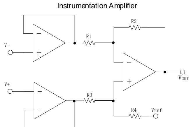
Figure 6. Instrumentation Amplifier
