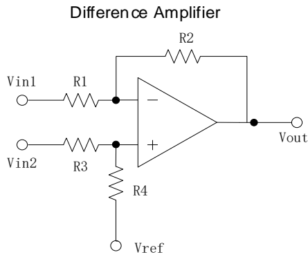
Figure 4. Differential Amplifier
