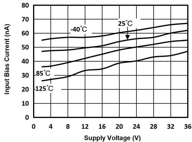
Input Bias Current vs Supply Voltage
