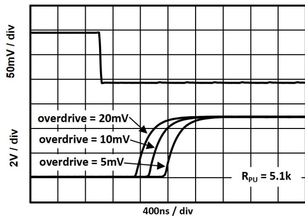
Response Time-Negative Transition
