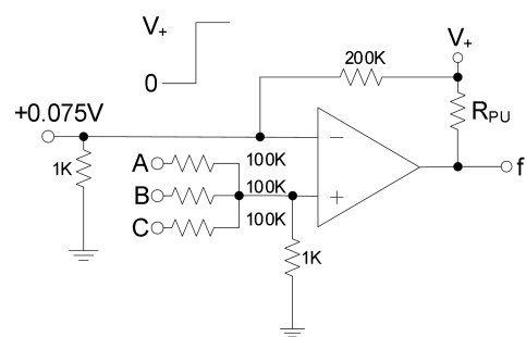
OR Gate
