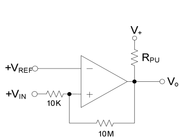
Non-Inverting Comparator with Hysteresis
