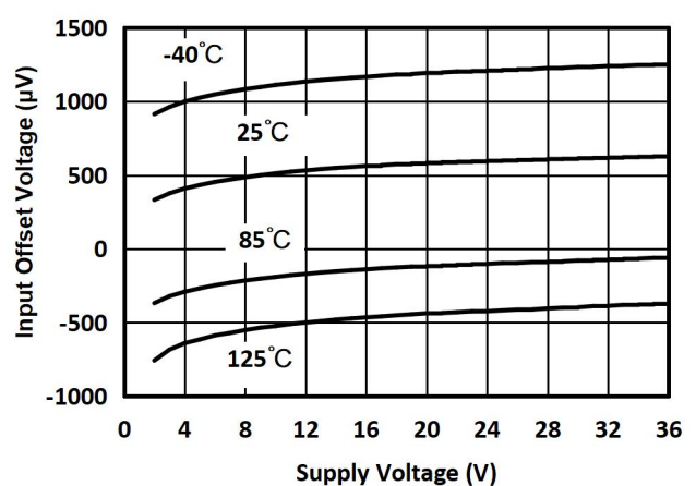
Input Offset Voltage vs Supply Voltage
