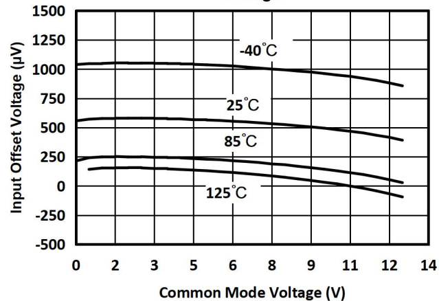
Input Offset Voltage vs Common Mode Voltage
