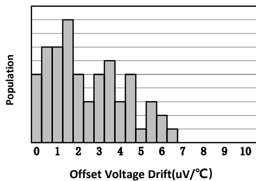
Offset Voltage Drift Magnitude Production Distribution
